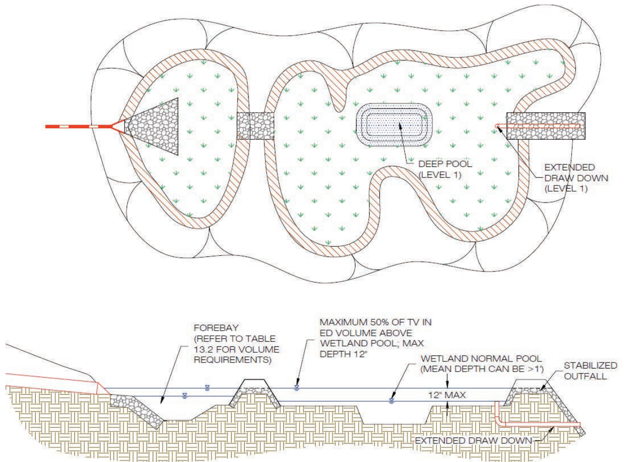
Figure 4: Constructed Wetland Plan and Cross Section.
