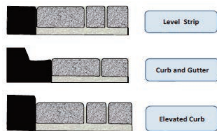
Figure 12: Examples of perimeter edge restraints (Source: NCDENR).
