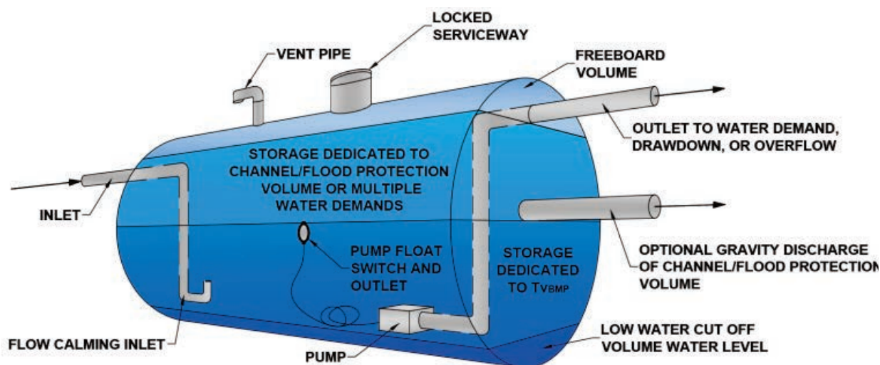
Figure 12: Tank Design 2 Storage Associated with Treatment, Channel Protection and Flood Volume (Source: VADCR, 2013).
