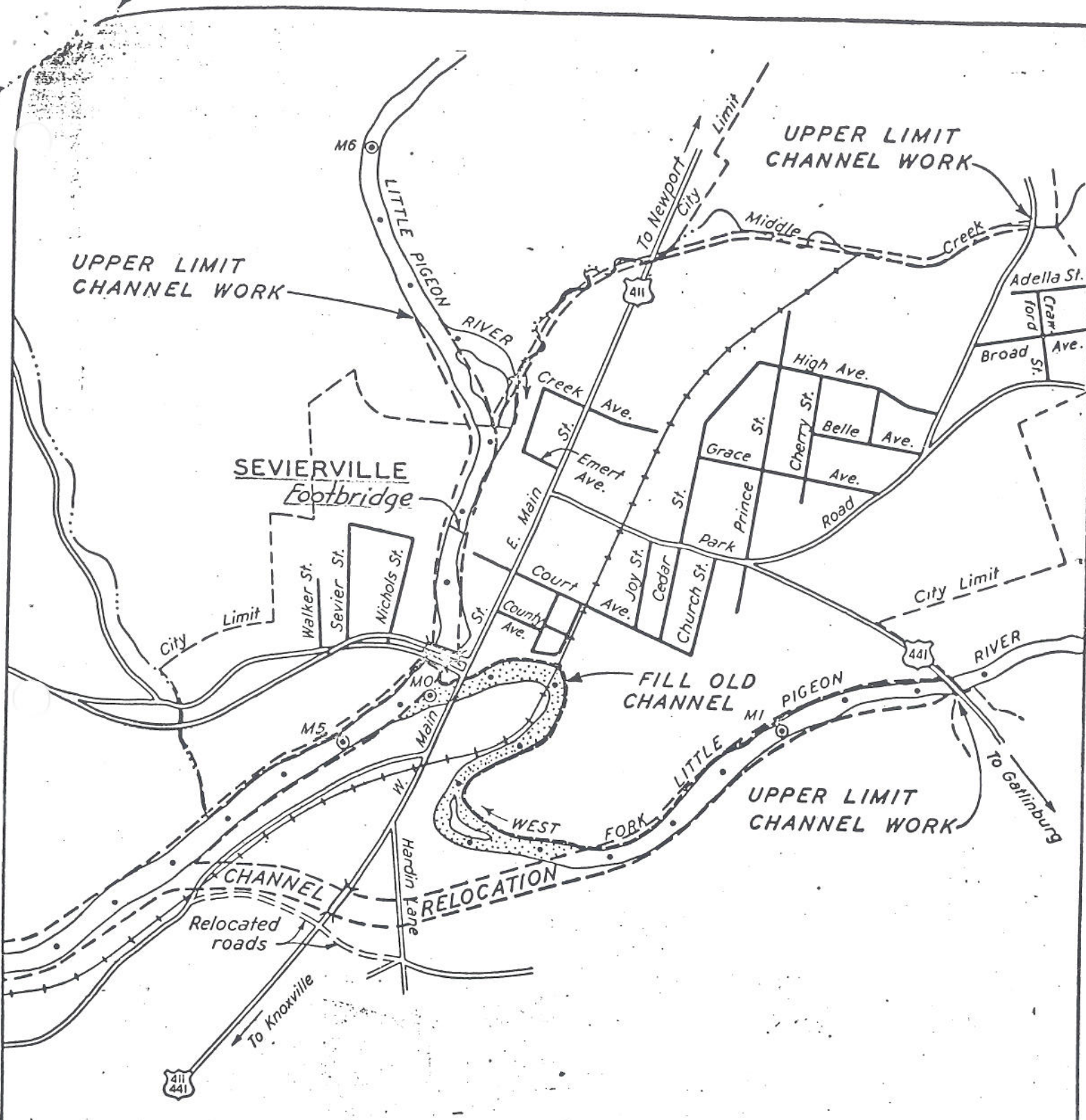
LITTLE PIGEON RIVER AND W. FORK LOCATION MAP FOR BRIDGE ABANDONMENT SEVIERVILLE, TENN. TENNESSEE VALLEY AUTHORITY DIVISION OF WATER CONTROL PLANNING EXHIBIT A
